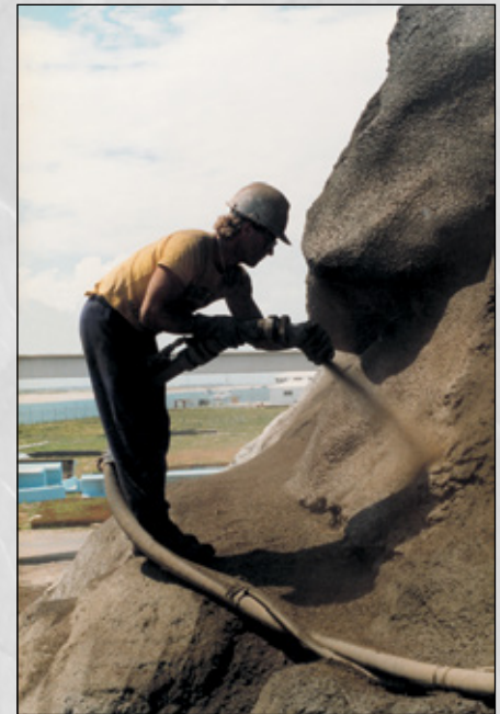
Forming the concrete with a concrete sprayer
