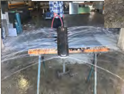
Front View with water - spraying under pressure
